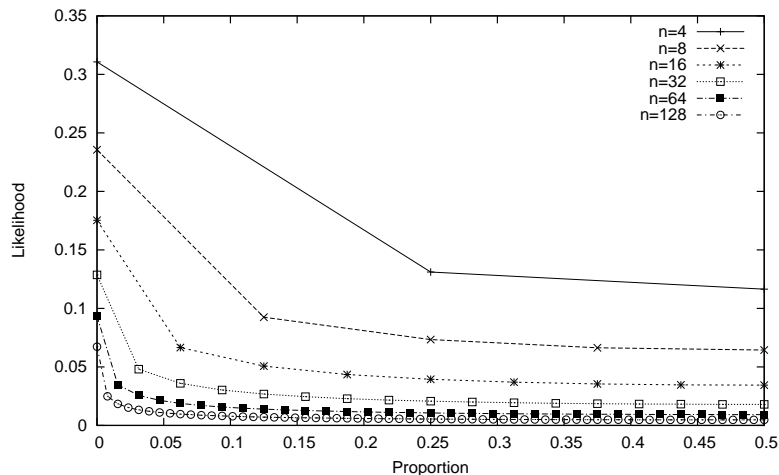
Figure 2: NML distribution for K=2 , different n .
