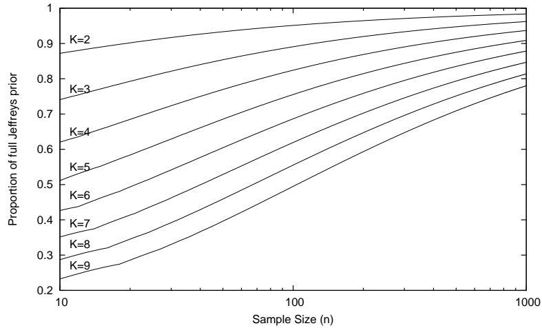
Figure 4: Proportion of Jeffreys prior in NML for the multinomial model.
