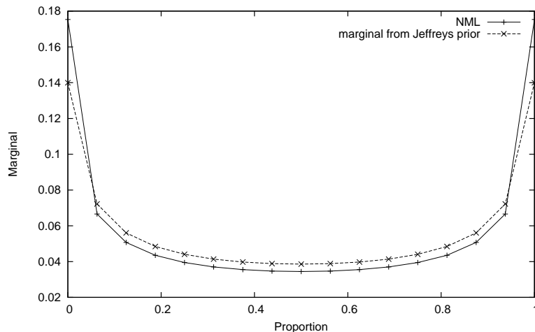
Figure 3: Jeffreys prior versus NML as P(\hat{\theta}|n = 16, M) for binomial.
