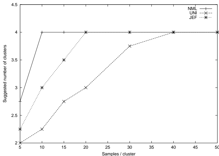
Figure 6: An example of the behavior of different clustering scores in the task of finding a four cluster data partitioning, as function of sample size per cluster.
