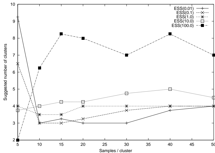
Figure 7: An example of the behavior of different ESS clustering scores in the task of finding a four cluster data partitioning, as function of sample size per cluster.
