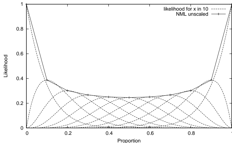
Figure 1: Likelihood curves for K=2 , n=10 .
